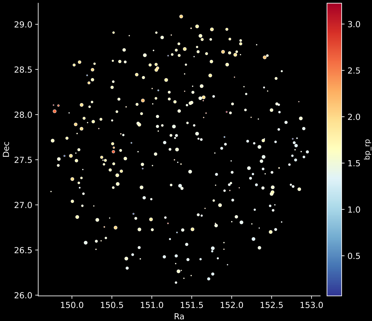
APOGEE DR17 Field: [160-24_btx] Stars: 312
