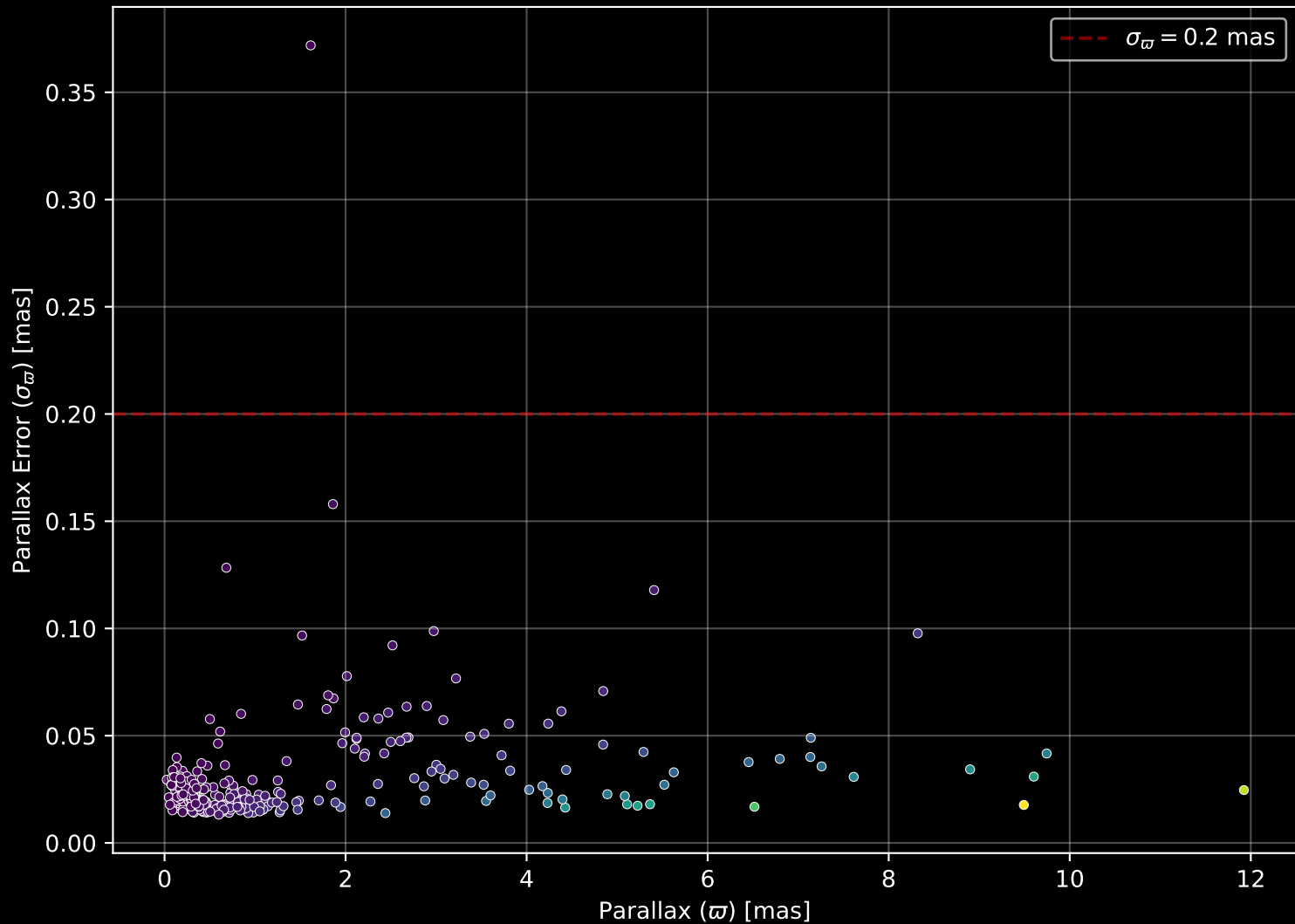
APOGEE DR17 Field: [160-24_btx] Parallax Quality (n= 312)
