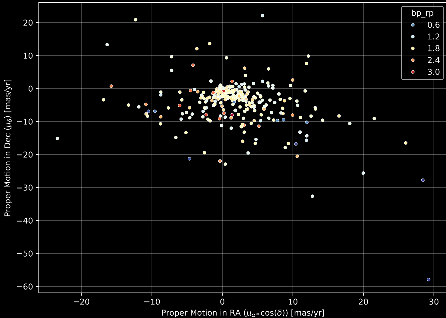
APOGEE DR17 Field: [160-24_btx] Proper Motion Diagram (n= 312)
