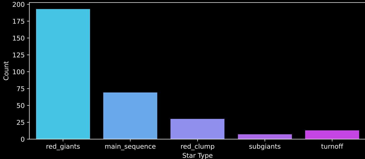
APOGEE DR17 Field: [160-24_btx] Count plot of Star Type
