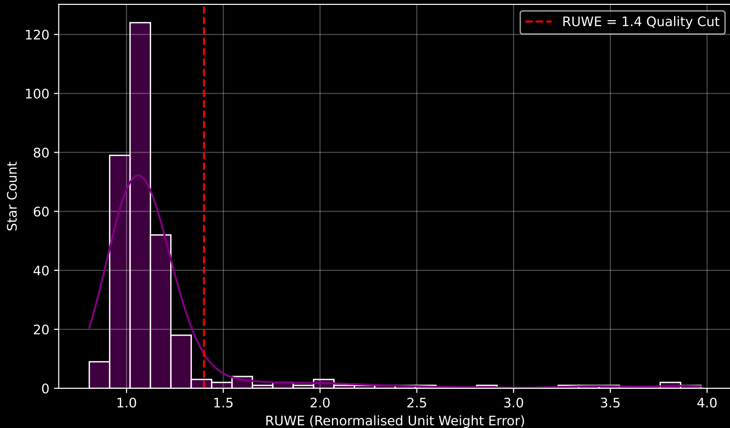
GAPOGEE DR17 Field [160-24_btx] RUWE Distribution (n= 310)
