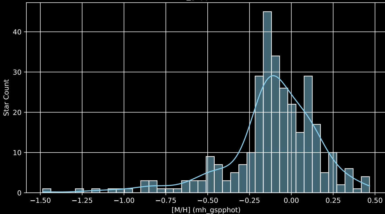
APOGEE DR17 Field: [160-24_btx [M/H] (mh_gspphot) (n= 310)
