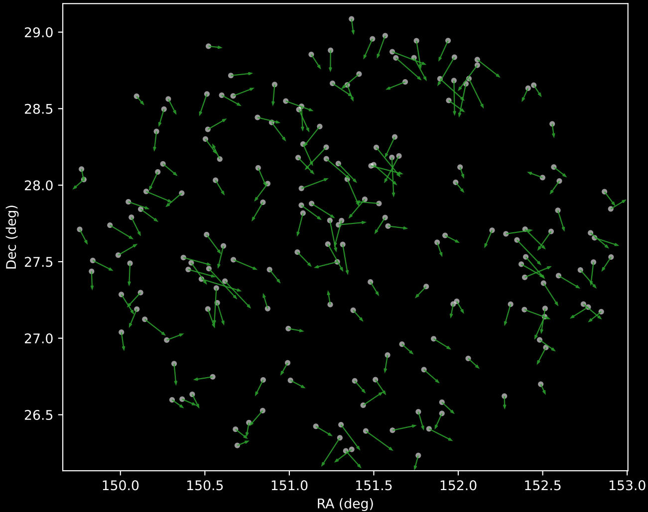
APOGEE DR17 Cluster 4 Proper Motion Vectors (n=185)
